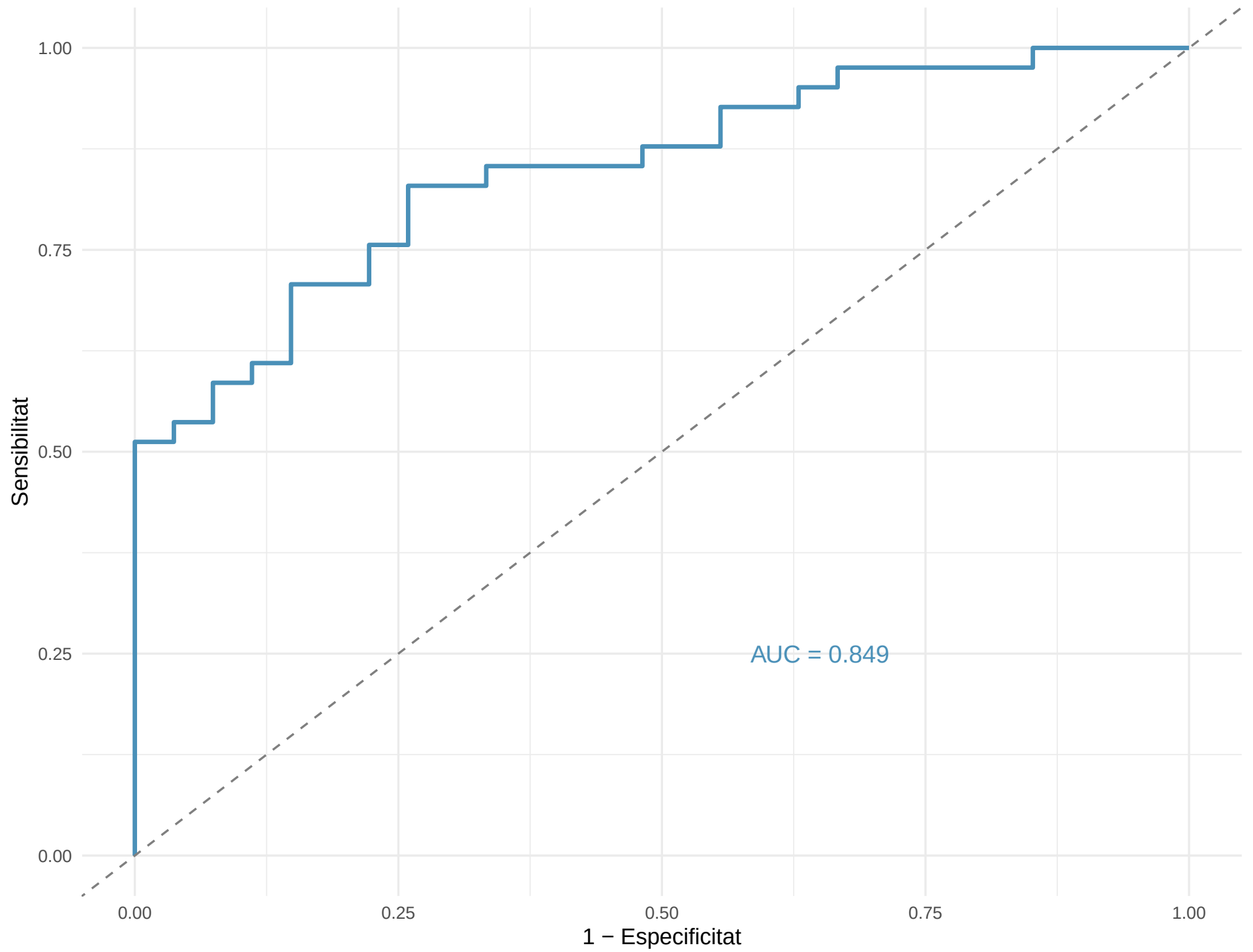
Corba ROC — SVM-RBF (test)
